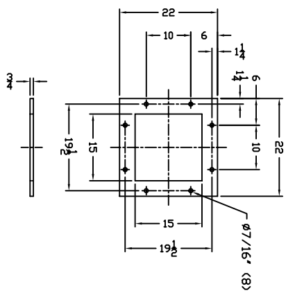
DISCHARGE FLANGE DETAIL 3/8" MS. SCALE 211
